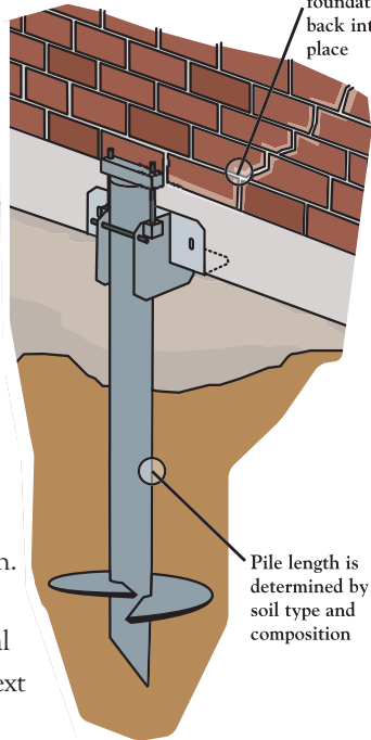
AF&R's Patented Articulating Bracket
